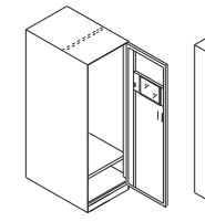
右手开门 左手开门 Wardrobe (Left/Right) 衣柜 (左/右) W400x D600 x H1170 W400x D600 x H1250 W400x D600 x H1260
