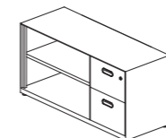
Fixed Return Combination Cabinet w/ Open Shelf & 2 Drawers 固定组合边柜, 书架及两斗抽屉 W800 - W1600 x D450 x H710 (except W1300, W1500)
