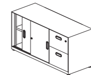
Fixed Return Combination Cabinet w/ Sliding Door & 2 Drawers W1100 - W1600 x D450 x H710 (except W1300, W1500)
