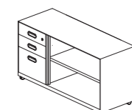
Mobile Return Combination Cabinet w/ Open Shelf & 3 Drawers 活动组合边柜, 书架及三斗抽屉 W800 - W1600 x D450 x H605 (except W1300, W1500)
