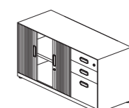
Fixed Return Combination Cabinet w/ Roller Door & 3 Drawers 固定组合边柜, 卷帘及三斗抽屉 W800 - W1600 x D450 x H710 (except W1300, W1500)
