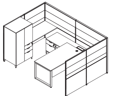
H Supervisor Desk, w/ Open Shelf & 2 Drawers + Cabinet for Panel w/ Single Swing Door & 3 Drawers 主管桌, 带空格柜,两抽屉 + 单掩门衣柜,带单掩门,三格抽屉
