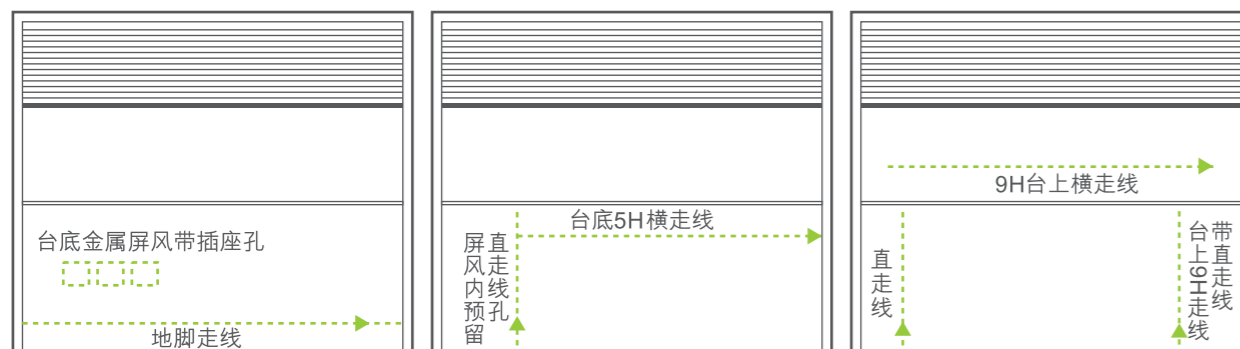
Cabling and socket cut outs at floor level
