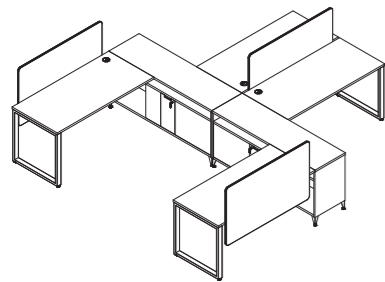
A Cluster of 4 workstations, Dual Cabinet w/ Open Shelf & Swing Door 四人工作位 双边矮柜,带掩门,空格柜
