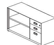
Fixed Return Combination Cabinet w/ Open Shelf & 3 Drawers 固定组合边柜, 书架及三斗抽屉 W800 - W1600 x D450 x H710 (except W1300, W1500)
