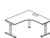
L-Shape Standard Desk L-型标准台 W1: 1400,1500,1600,1800 D1: 600,700,800 W2: 1400,1500,1600,1800 D2: 600,700
