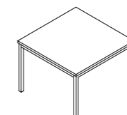
Coffee Table/茶几 W600 D600 H447
