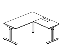
L-Shape Integrative Desk L-型组合台 W1: 1500,1600,1800 D1: 700,800 W2: 1500,1600,1800 D2: 600
