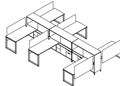
Cluster of 6 workstations, Dual Cabinet w/Open Shelf & Swing Door & 2 Drawers 六人工作站 双边高柜·带空格柜·单掩门·两抽屉
