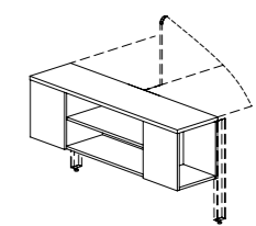
Three Sides Open Cabinet 三面开口柜 W: 1200,1400,1600 H: 360
