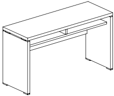
Training Table 条形训练桌 W1400 D500 H770 W1500 D500 H770
