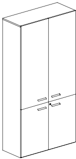
High Cabinet w/4 Wood Door 4 门高柜 (全木门) W800 D420 H2000 W1000 D420 H2000
