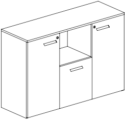
Low Cabinet w/2 Swing Doors, Open Shelf and Drawer 两掩门矮柜带空格及抽屉 W1200 D420 H800
