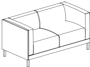
Sofa, Two-Seated 双人沙发 W1430 D730 H710
