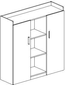
2 Swing Doors and Open Shelf Middle Cabinet 两掩门中柜 W1340 D420 H1382
