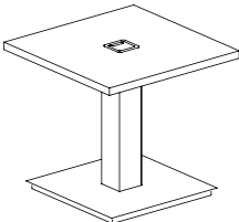
Meeting Table 洽谈桌 W800 D800 H745 W900 D900 H745 W1000 D1000 H745
