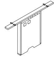
Intermediate Leg, with trunking 中间脚 · 带走线 W: 1000, 1200 H: 720
