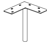
Short Leg, Corner Shared 矮脚·转角脚 W230 x D230 x H280
