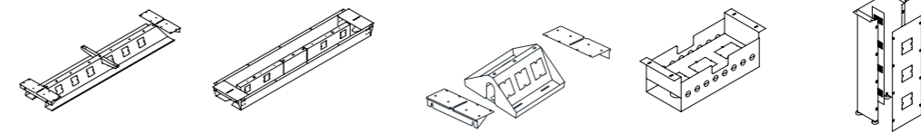
Standard Trunking 常规走线槽 Reinforce Trunking 加高走线槽 Basic Trunking 基本款走线槽 Socket Box 插座线盒 Vertical Trunking 垂直上线槽
