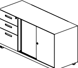
Metal Mobile Sliding Door Cabinet w/3 Drawers (L/R) 3 抽钢制活动移门边柜 (左/右) W: 1000,1100,1200 D: 450 H: 605
