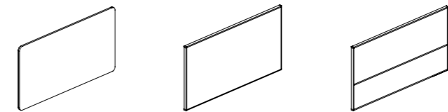
Frameless Screen 无框屏风 W: 626,726,826,1200,1400,1600 H: 784 Framed Screen (w/o Press Bar) 有框屏风 (无压条) W: 626,726,826,1200,1400,1600 H: 784 Framed Screen (w/Press Bar) 有框屏风 (有压条) W: 626,726,826,1200,1400,1600 H: 784
