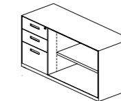
Fixed Metal Open Shelf Cabinet w/3 Drawers (L/R) 3 抽钢制固定空格边柜 (左/右) W: 800,900,1000,1100,1200 D: 450 H: 710
