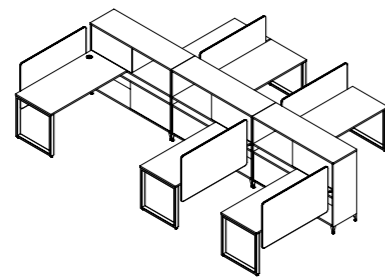
Cluster of 6 workstations, Dual Cabinet w/Open Shelf 六人工位 双边高柜·带空格柜
