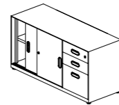
Fixed Metal Sliding Door Cabinet w/ 3 Drawers 3 抽钢制固定移门边柜 W: 1100-1600 D: 450 H: 710 (Except W1300, W1500)
