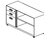
Metal Mobile Open Shelf Cabinet w/ 3 Drawers 3 抽钢制活动空格边柜 W: 800-1600 D: 450 H: 605 (Except W1300, W1500)
