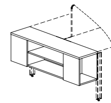
Three Sides Open Cabinet 三面开口柜 W: 1200,1400,1600 H: 360
