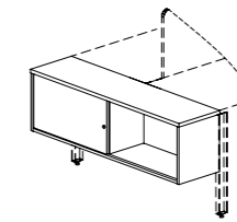
Single Sliding Cabinet 单趟门柜 W: 1200,1400,1600 D: 360
