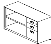
Fixed Metal Open Shelf Cabinet w/ 3 Drawers 3 抽钢制固定空格边柜 W: 800-1600 D: 450 H: 710 (Except W1300, W1500)
