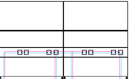
Cabling and Socket Above Work Surface with Vertical Internal Raceway 台底 5H 横走线
