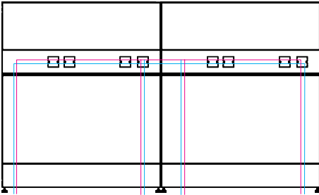
Cabling and Socket Under Work Surface with Vertical Internal Raceway 台上横走线
