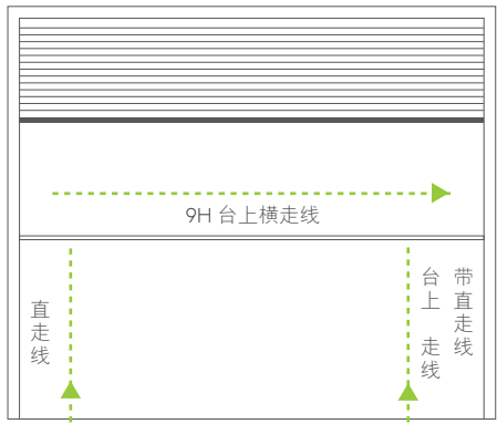
Cabling and Socket Above Work Surface with Vertical Internal Raceway ( Only A50)
