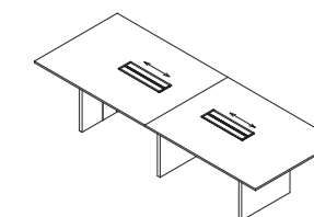
Rectangular Shape Conference Table, with Socket Channel 长方形会议桌,带走线槽
