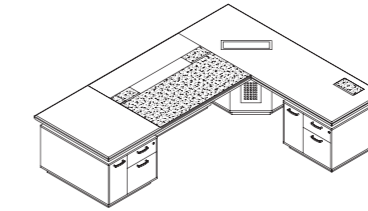
Executive desk w/ pedestal, extension & LCD lifter 大班桌，连抽屉柜及翻台，LCD升降台
