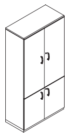
High cabinet, wooden doors without coat hanger 高柜·木门·无挂衣架 MYC2010W ( ) - W1000 x D470 x H2030
