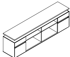
LOWER CABINET W/2 SETS OF DRAWERS W/PLATE 矮柜带双边抽屉·带柜顶板 W2200 D500 H745 W2400 D500 H745
