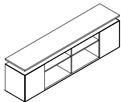
LOWER CABINET W/2 SWING DOORS W/PLATE 矮柜带双掩门·带柜顶板 W2200 D500 H745 W2400 D500 H745
