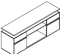
LOWER CABINET W/SINGLE SET OF DRAWER W/PLATE 矮柜带单边抽屉·带柜顶板 W1200 D500 H745
