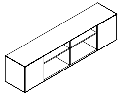
LOWER CABINET W/2 SWING DOORS 矮柜带双掩门 W2200 D500 H630 W2400 D500 H630
