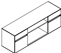
LOWER CABINET W/ SINGLE SET OF DRAWER 矮柜带单边抽屉 W1200 D500 H630
