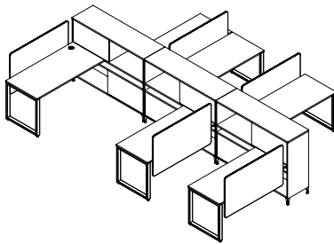
Cluster of 6 workstations, Dual Cabinet w/Open Shelf 六人工位 双边高柜，带空格柜
