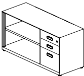
Fixed Metal Open Shelf Cabinet w/ 3 Drawers 3 抽钢制固定空格边柜 W: 800-1600 D: 450 H: 710 (Except W1300, W1500)
