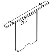
Intermediate Leg, with trunking 中间脚 · 带走线 W: 1200, 1200 H: 720
