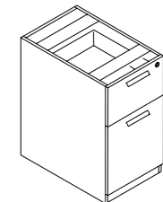
Fix Pedestal (2 drawers) 两抽固定柜 W: 380 D: 600,700 H: 720
