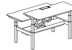
Height-adjustable Double Bench with Horizontal Trunking 双边升降共享台·带横走线槽 W: 1400, 1500, 1600 D: 1400, 1600 H: 635 - 1285
