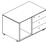
Mobile Pedestal w/ Open Shelf, 3 drawers 矮柜带空格, 三个抽屉 W900 x D550 x H600
