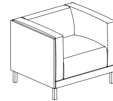
Sofa, One-Seated 单人沙发 W840 D730 H710
