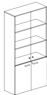
High Cabinet w/Glass and Wood Door 4门高柜(上玻璃·下木门) W800 D420 H2000 W1000 D420 H2000
