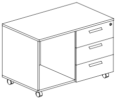
Mobile Pedestal w/3 Drawers and Open Shelf 活动柜桶带三抽屉及空格 W900 D550 H600
