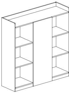
Single Sliding Door Middle Cabinet 单趟门中柜 W1340 D420 H1382
