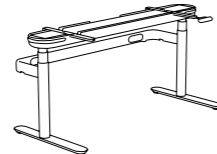
HAD Adjustable Leg 独立升降脚架 W: 1400,1500,1600,1800 H: 600, 700
