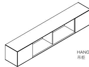
HANGING CABINET 吊柜 W1800 D400 H420
