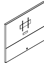
WORK WALL UNIT W/TV MOUNT 背景墙带电视架 W2400 D80 H2000
