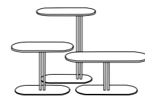
Oblong Occasional Table 椭圆盘脚休闲桌椭圆台面 W900/1200 D400 H500/650 Oblong Desktop w/2 Side Column Base 双柱偏边底座 W900 D400 H1050
