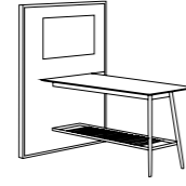
2 Legs High Table 两脚高桌 W1980 D950 H1050
