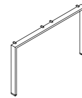
25 x 50 50 Square End Leg, Open 50 方形开口边脚 W: 1200, 1400 H: 720
