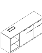
Return Cabinet A 边柜 A W1700 D500 H630
