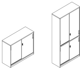
W700/800/900/1000/1100/1200 D400/450 H745/900/1145/1300/1700/2100 (Embedded Handle) (内嵌拉手)
