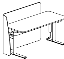
Side Straight Screen (for HAD) (L/R) 侧边直形屏风 (HAD 独立台专用) (左 / 右) W: 1200 D : 1100,1200
