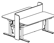
S Centert Screen (Connected) (for HAD) (L/R) S形中间连接屏风 (HAD 独立台专用) (左 / 右) W: 1400,1500,1600,1800 D : 1100,1200
