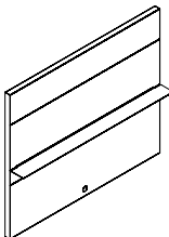
WORK WALL UNIT W/METAL SHELIVING 背景墙带金属架 W1800 D80 H2000 W2200 D80 H2000 W2400 D80 H2000
