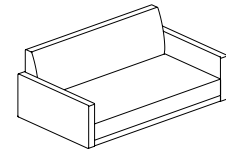
2-Seater Sofa, Two Arms 两人位沙发·两扶手 W1100 x D700 x H465 W1400 x D700 x H465 W1500 x D700 x H465 W1600 x D700 x H465
