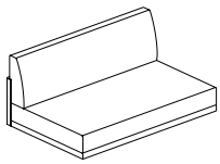
2-Seater Sofa, Armless 两人位沙发·无扶手 W1100 x D700 x H465 W1400 x D700 x H465 W1500 x D700 x H465 W1600 x D700 x H465
