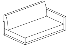
2-Seater Sofa, Left Arm 两人位沙发·左扶手 W1100 x D700 x H465 W1400 x D700 x H465 W1500 x D700 x H465 W1600 x D700 x H465
