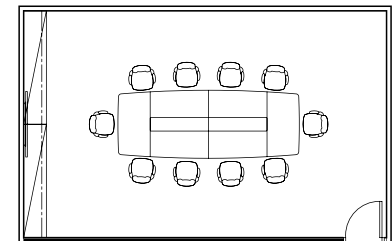
CONFERENCE TABLE 会议桌 LOWER CABINET W/2 SETS OF DRAWERS W/PLATE 矮柜带双边抽屉，带柜顶板 CHAIR
