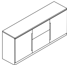
Low Cabinet, Wooden Doors w/Drawers 矮柜带木门抽屉 W1800 D470 H750
