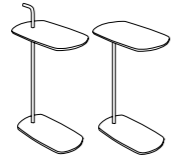
Side Table w & w/o Handle W320 D550 H650 W320 D550 H800
