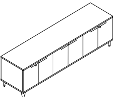
W1200/1500/1800 D450 H500
