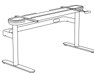
Fixed Leg for Single Desk W : 1400,1500,1600,1800 H : 600, 700
