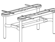
Fixed Leg for Bench W : 1400,1500,1600,1800 H : 600, 700
