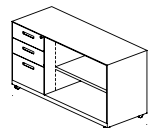
Fixed Metal Open Shelf Cabinet w/3 Drawers (L/R) 3 抽钢制固定空格边柜 (左/右) W800/900/1000/1100/1200 D450 H710
