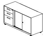
Fixed Metal Sliding Door Cabinet w/3 Drawers (L/R) 3 抽钢制固定移门边柜 (左/右) W1000/1100/1200 D450 H710
