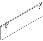
MFC Modesty Panel Hang on Bar 三聚氰胺板前挡板·横杆悬挂 W: 940, 1140, 1240, 1340 T: 16 H: 350
