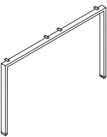
25 x 70 70 Square End Leg, Open 70 方形开口边脚 W: 1200, 1400 H: 720
