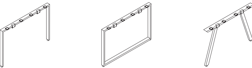
50 x 25 50 Square End Leg, Open (50A) 50 方形开口脚 W: 1200, 1400 H : 720 50 x 25 50 Square End Leg, Closed (50B) 50 方形封口脚 W: 1200, 1400 H : 720 60 x 30 60 Trapezoid End Leg, Open (60C) 60 梯形开口脚 W: 1200, 1400 H : 720
