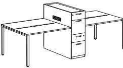
Double-sided Bench with High Cabinet for 4 Staffs 对座台带高柜 - 4 人 W: 2800, 3200, 3400 D: 1232, 1432 BH: 745 CH: 1100
