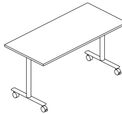
Unfoldable Training Table with Castors 非折叠培训台带脚轮 W: 1200, 1400, 1500, 1600 D: 600, 700 H: 755
