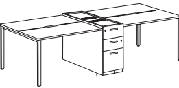
Double-sided Bench with Low Cabinet for 4 Staffs 对座台带矮柜 - 4 人 W: 2800, 3200, 3400 D: 1232, 1432 BH: 745 CH: 780
