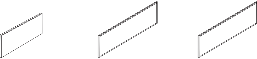
Desktop Frameless Screen (Half Width) – Fabric 桌上 框屏风 (半宽) - 布屏风 W : 1000, 1200, 1300 H : 400 T : 20 Desktop Screen w/frame (Full Width) – Fabric 桌上有框屏风 (全宽) - 布屏风 W : 1200, 1400, 1500 H : 380 T : 30 Desktop Tackable Screen w/frame (Full Width) – Fabric 桌上有框针板屏风 (全宽) - 布屏风 W : 1200, 1400, 1500 H : 380 T : 30
