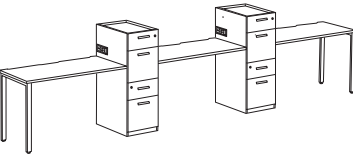
Single-sided Bench with High Cabinet for 3 Staffs 单边台带高柜 - 3 人 W: 4400, 5000, 5300 D: 616, 716 BH: 745 CH: 1100
