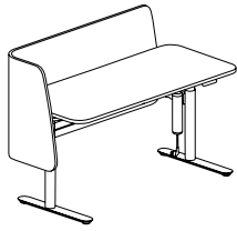
L Long Wave Screen (for HAD) (L/R) W : 1400,1500,1600,1800 D : 1100,1200
