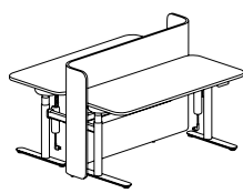
S Centert Screen (Connected) (for HAD) (L/R) W : 1400,1500,1600,1800 D : 1100,1200
