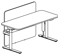
Center Straight Screen (for HAD) W : 1400,1500,1600,1800 D : 1100,1200
