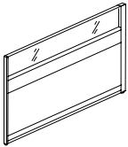
Panel, w/Transparent Tile (Floor Standing) 落地屏风带透明风格 W: 600,700,800,900,1000,1200,1400, 1500,1600 H: 1100,1207,1507,1657
