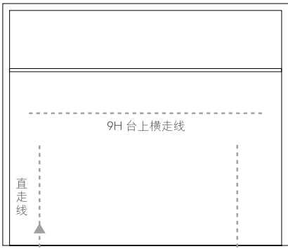
Cabling and Socket Above Work Surface with Vertical Internal Raceway ( Only E50)
