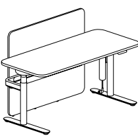
Center Straight Screen (for HAD) 中间直屏风 (HAD 独立升降台专用) W: 1400,1500,1600,1800 D : 1100,1200
