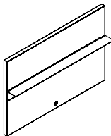
WORK WALL UNIT W/METAL SHELVING 背景墙带金属架 W1800 D80 H1200 W2200 D80 H1200 W2400 D80 H1200
