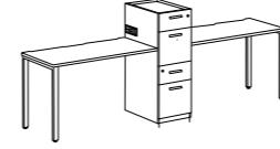
Single-sided Bench with High Cabinet for 2 Staffs 单边台带高柜 - 2人 W: 2800, 3200, 3400 D: 616, 716 BH: 745 CH: 1100
