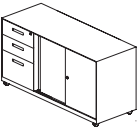
Fixed Metal Sliding Door Cabinet w/ 3 Drawers (L/R) 3 抽钢制固定移门边柜 (左/右) W1000/1100/1200 D450 H710
