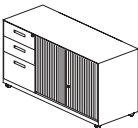
Fixed Metal Roller Door Cabinet w/ 3 Drawers (L/R) 3 抽钢制固定卷帘边柜 (左/右) W800/900/1000/1100/1200 D450 H710
