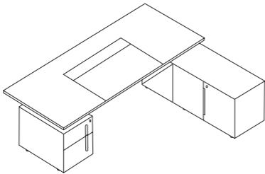
Executive Desk w/pedestal, return cabinet (w/slider door) W1800 D1880 H750 W2000 D1880 H750 W2200 D2000 H750 W2400 D2000 H750
