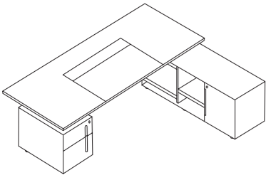
Executive Desk w/pedestal, return cabinet (w/CPU rack) W1800 D1880 H750 W2000 D1880 H750 W2200 D2000 H750 W2400 D2000 H750
