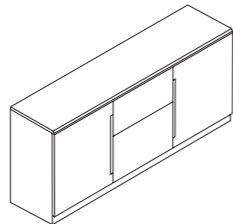
Low Cabinet, Wooden Doors w/Drawers W1800 D470 H750
