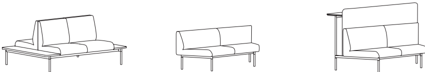
Double-side 2-Seated with 2 Side Table 双座双排沙发带边几 L/B 矮背：W1800 D1320 H760 H/B 高背：W1800 D1320 H840 Trapezoidal Sofa 切角沙发 L/B 矮背：W1870 D660 H760 H/B 高背：W1870 D660 H840 Trapezoidal Back Sofa with Back Screen and Bar Table 切角高背沙发带背板及吧台 W2285 D1035 H1200
