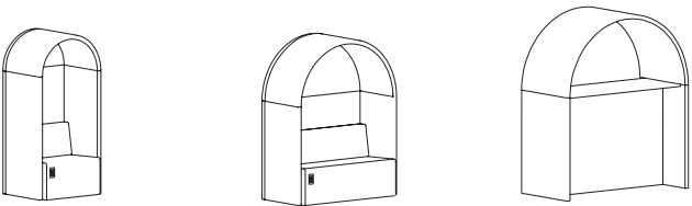
1-Seater Cabin, w/ or w/o Socket 拱门形单座沙发，不带或带 电源 W920 D750 H1900 2-Seater Cabin, w/ or w/o Socket 拱门形双座沙发，不带或带 电源 W1460 D750 H1900 Bar Counter 拱门形吧台 W1910 D910 H2100
