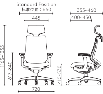
High Back Chair with Headrest and Armrest 高背座椅带头靠及扶手
