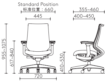
High Back Chair with Armrest 高背座椅带扶手
