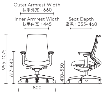
High Back Chair with Armrest 高背座椅带扶手
