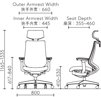
High Back Chair with Headrest and Armrest 高背座椅带头靠及扶手
