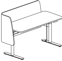
L Long Wave Screen (for HAD) (L/R) W : 1400,1500,1600,1800 D : 1100,1200
