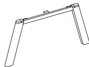
A-Shape Leg Single Bench Double Bench W: 600, 700, 750 W: 1200, 1400, 1500 H: 725 H: 725
