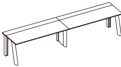
Single Bench w/Straight Mid-leg and Cable Cover for 2 People W: 2400^, 2800, 3000, 3200, 3600 D: 800, 900, 950 H: 725
