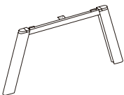
A-Shape Leg Single Bench Double Bench W: 600, 700, 750 W: 1200, 1400, 1500 H: 725 H: 725
