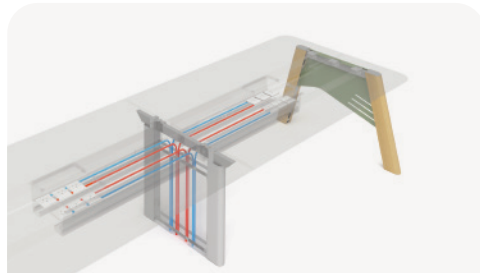
Straight Mid-leg Power and Data Cable Management
