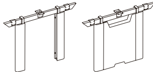
Straight Leg w/or w/o Cable Cover Single Bench Double Bench W: 600, 700, 750 W: 1200, 1400, 1500 H: 725 H: 725
