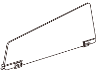
Asymmetric Frameless Screen - Fabric, PET, MFC W: 1200, 1400, 1500, 1600, 1800 H: 455
