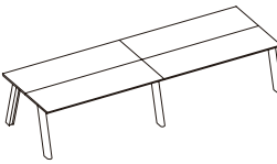
Double Bench w/A-Shape Mid-leg for 4 People W: 2400^, 2800, 3000, 3200, 3600 D: 1200, 1400, 1500 H: 725
